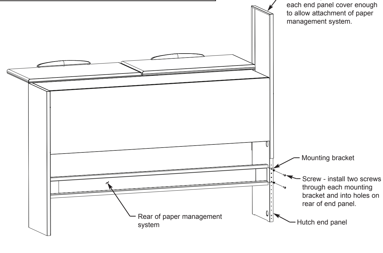
Illustration 2. Attach Paper Management System to Hutch:
