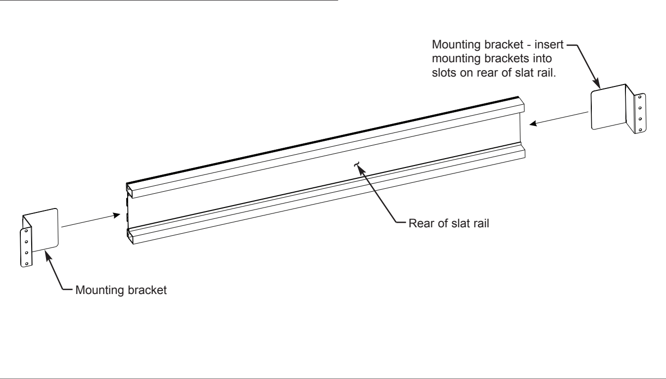
Illustration 2. Attach Paper Management System to Hutch:
